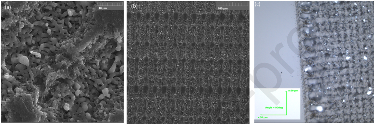
Fig 3 (a) SEM image of the ablation pattern with dense microstructures (b) SEM image of the glass wafer with highly ordered ablation pattern (c) Optical profilometer image of microcracks formed on the glass wafer due to thermomechanical stress at wrong laser micro structuring parameters
