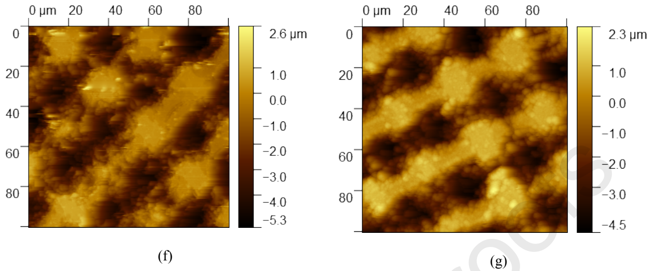
Fig 5 (a) Surface morphological features of the glass wafers after microstructuring (b) Cross-section SEM view of the cross-hatching pattern (c) & (d) Morphology of copper-plated glass wafers on the patterns shown at different scan areas (e) Cross-sectional image of the plated copper on the glass with thickness scale (f) 2D AFM image of the micromachined glass wafer (g) 2D AFM image of the micromachined glass wafer with copper electroplated.
